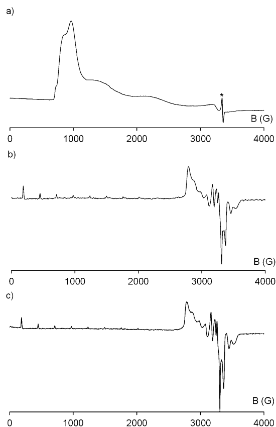
Figure 3. Top: X-Band EPR spectrum for complex [(CAAC)_2Fe]BAR_{24}^F ( 3 ) in a 2-methyltetrahydrofuran glass at 10 K; * denotes a trace impurity. Middle: X-Band EPR spectrum for complex [(CAAC)_2Co] ( 7 ) in a toluene glass at 10 K. Bottom: X-Band EPR spectrum for complex 7 in a toluene glass at 77 K.
